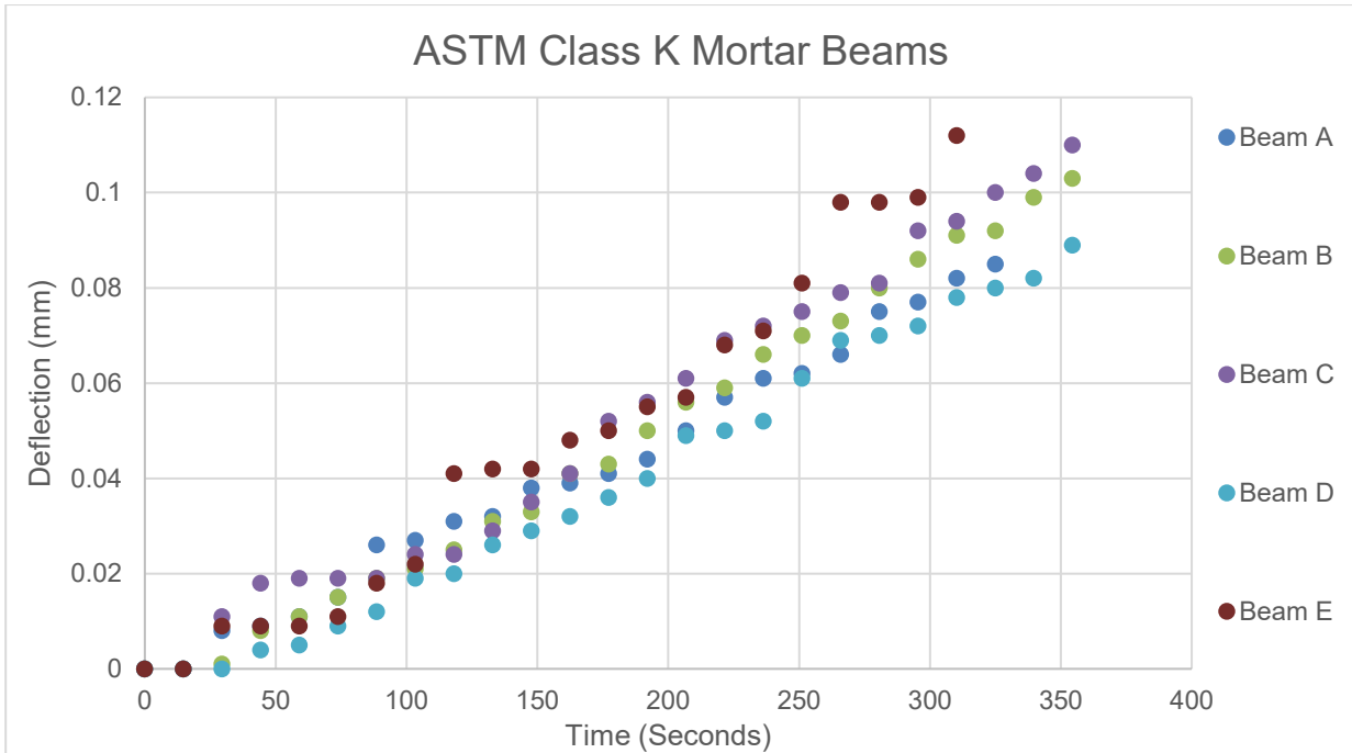
Graph 4.5: Results of Young's Modulus for ASTM Class K mortar beams
