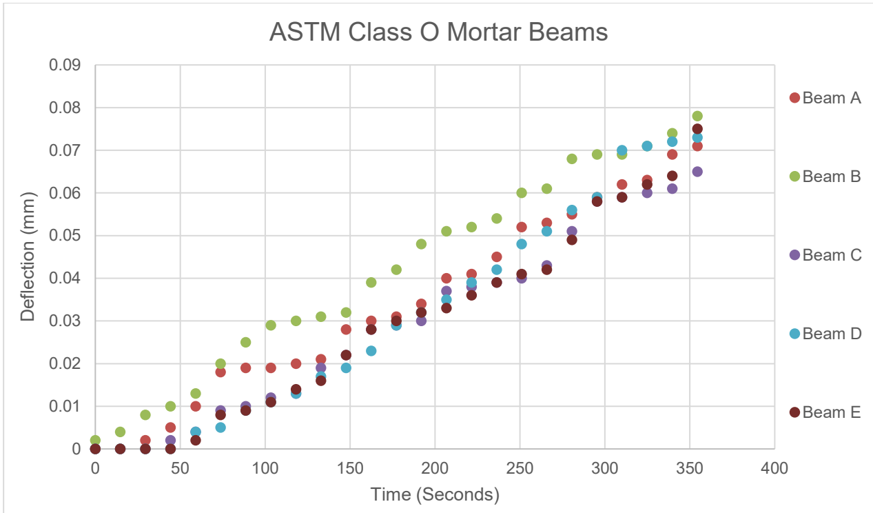
Graph 4.4: Results of the Young's Modulus for ASTM Class O mortar beams
