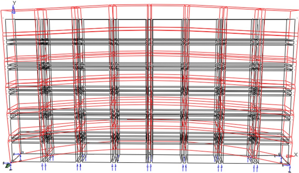
Figure 5.7: Outline of finite element wall panel with displacement added
