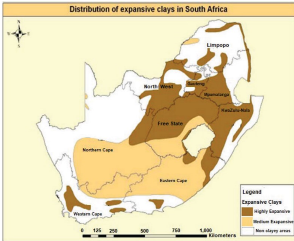
Figure 2.1: Distribution of expansive clay in South Africa
