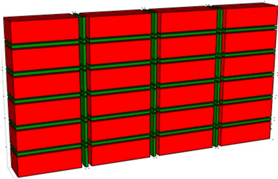
Figure 5.4: Finite element wall panel of initial model in a stack bond pattern
