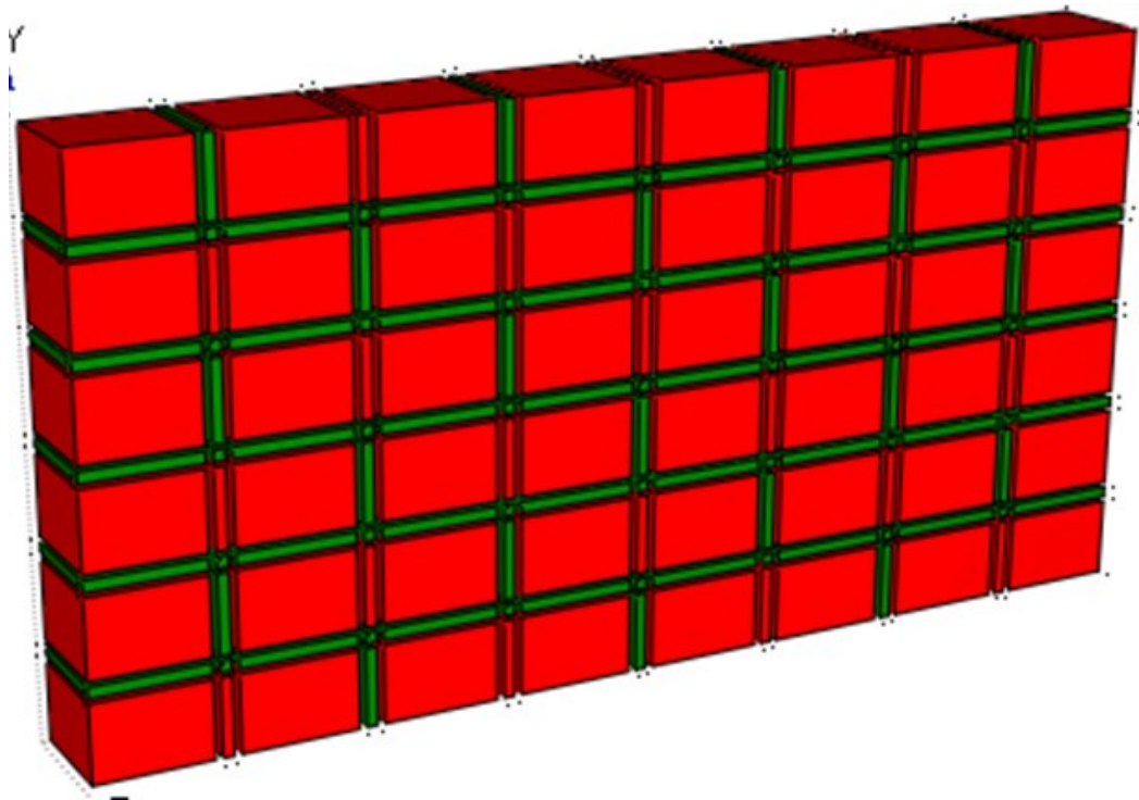
Figure 5.6: Finite element wall panel designed using the first mesh refinement
