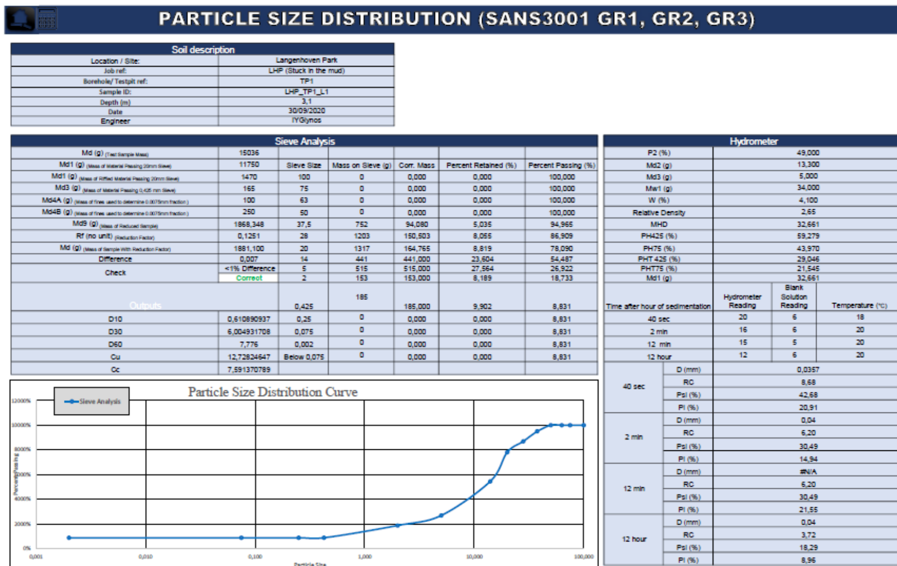
Figure 36 – Particle size and hydrometer worksheet
