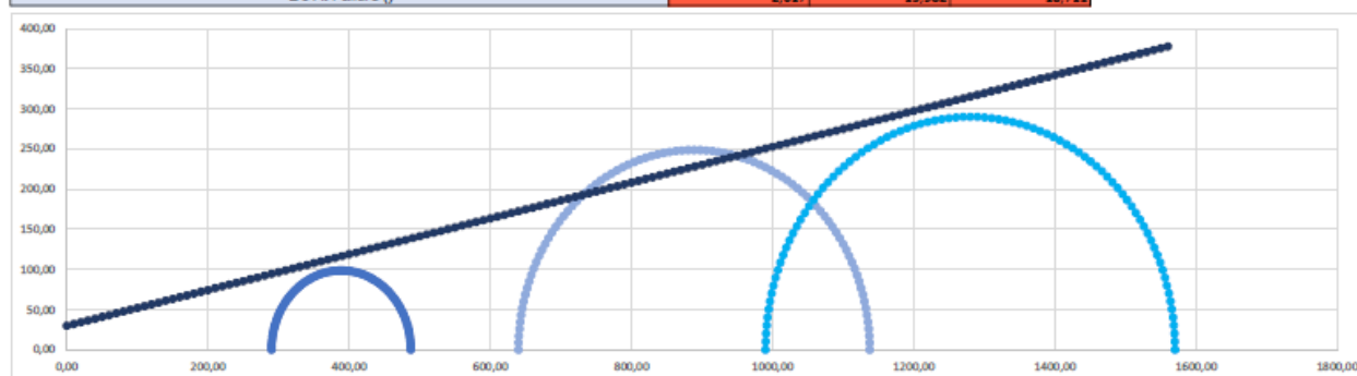
Figure 56 – Triaxial Worksheet
