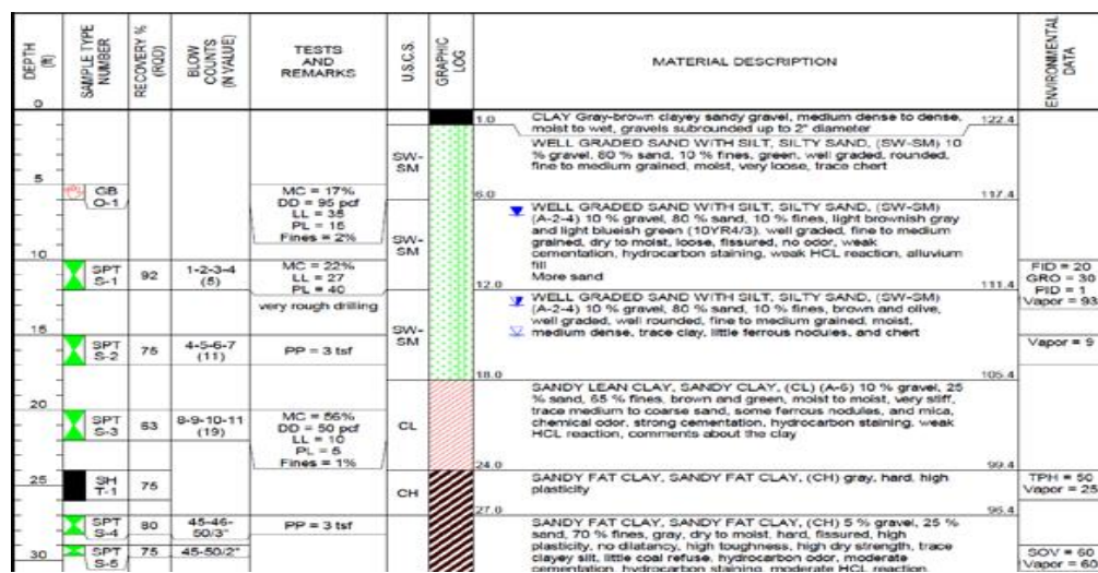
Figure 24 - Subsurface data of gINT
