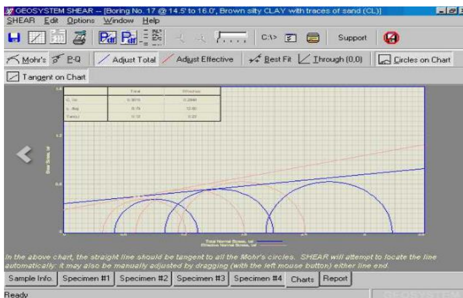
Figure 20 - GEOSYSTEMS Shear
