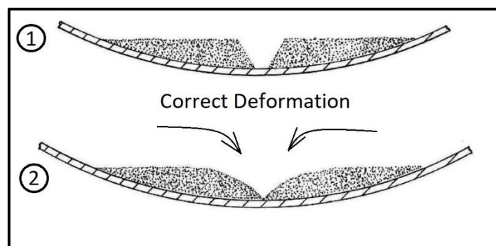
Figure 2-5: Correct deformation of soil in cup
