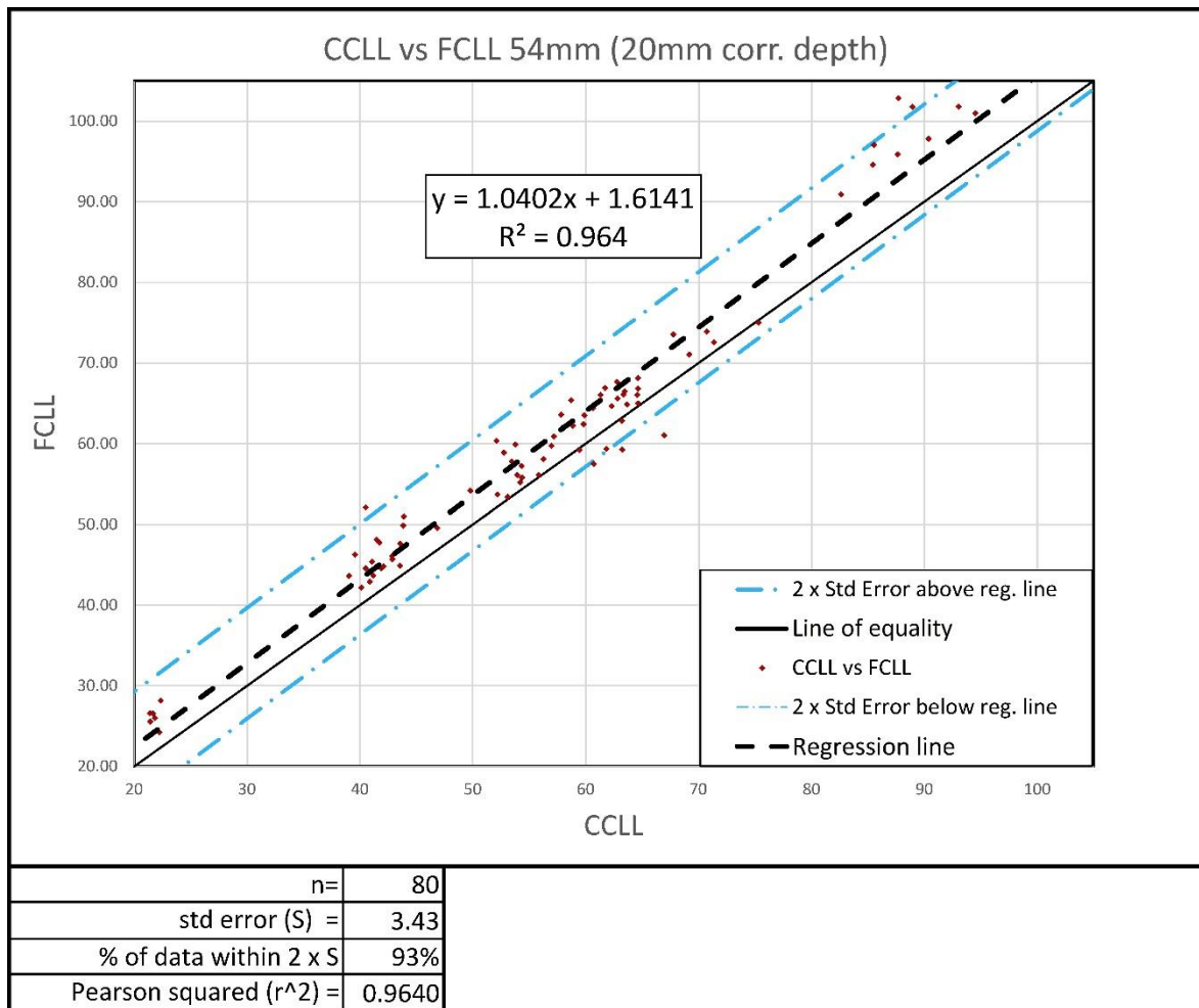
Figure 4-7: Linear reg. of CCLL vs FCLL 54 at 20mm penetration.
