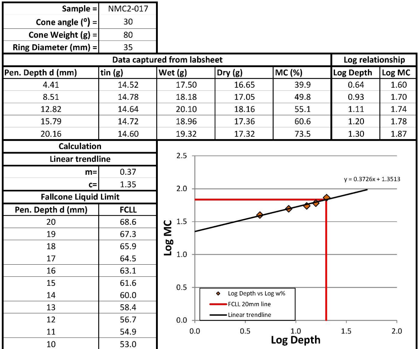
Figure 3-19 Calculation of the FCLL
